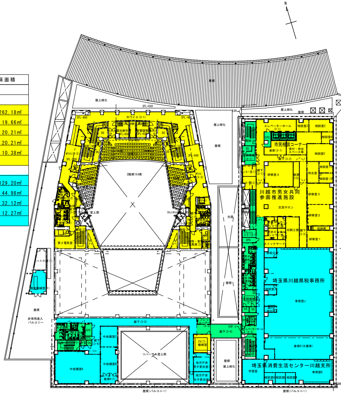
3階平面図 Scale:1/500
